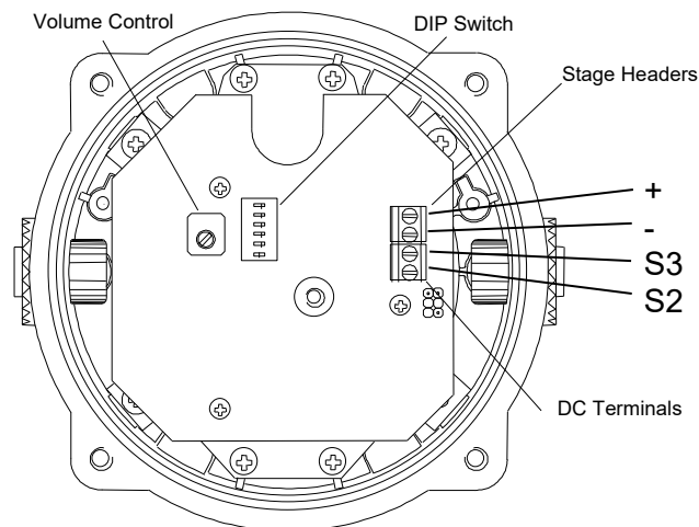
Fig. 6 DC Terminals
