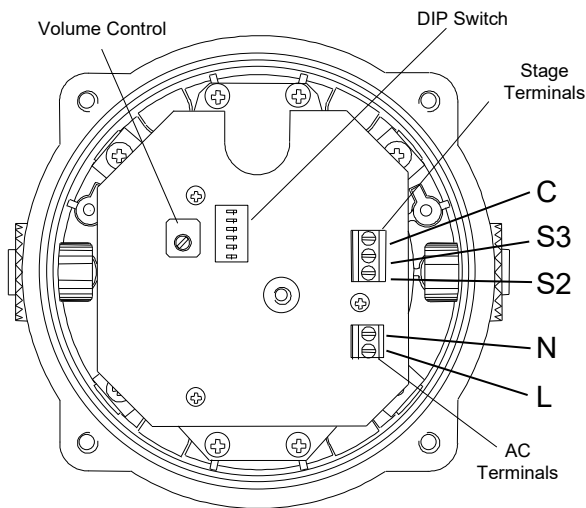
Fig. 4 AC Terminals
