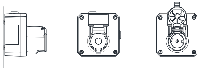
Fig 1 Wall Mounting
