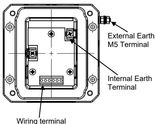
Fig 3 Earth terminals
